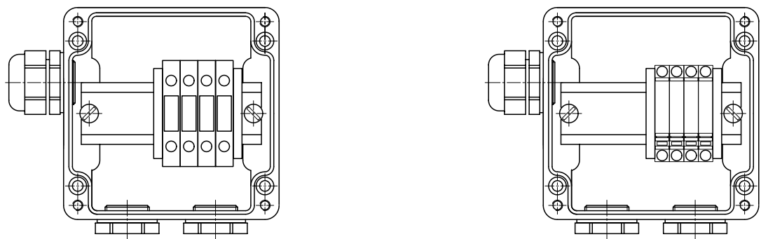
JB2212-223-2xxxx box with screw clamp (left) and push-in (right) terminal block. Number of terminals and cable glands may vary.
